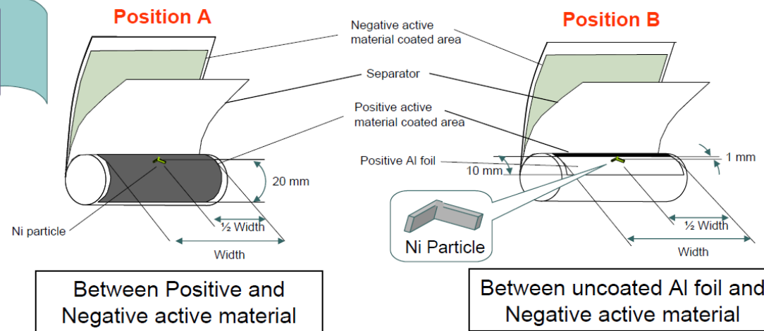
The trigger of the accident is the internal short-circuit between the positive electrode and negative electrode
